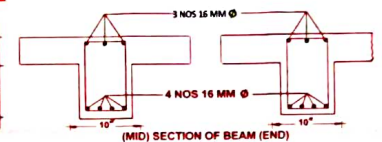
(MID) SECTION OF BEAM (END)
