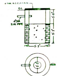
CIRCULAR SOAK WELL
